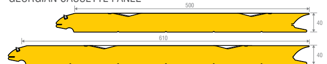
GEORGIAN CASSETTE PANEL
