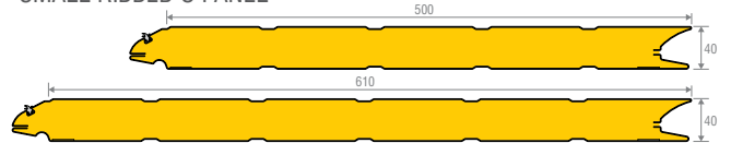
SMALL RIBBED U PANEL
