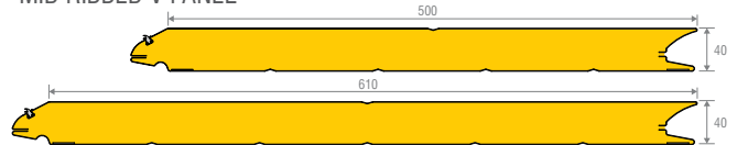
MID RIBBED V PANEL
