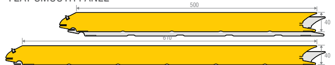
FLAT SMOOTH PANEL
